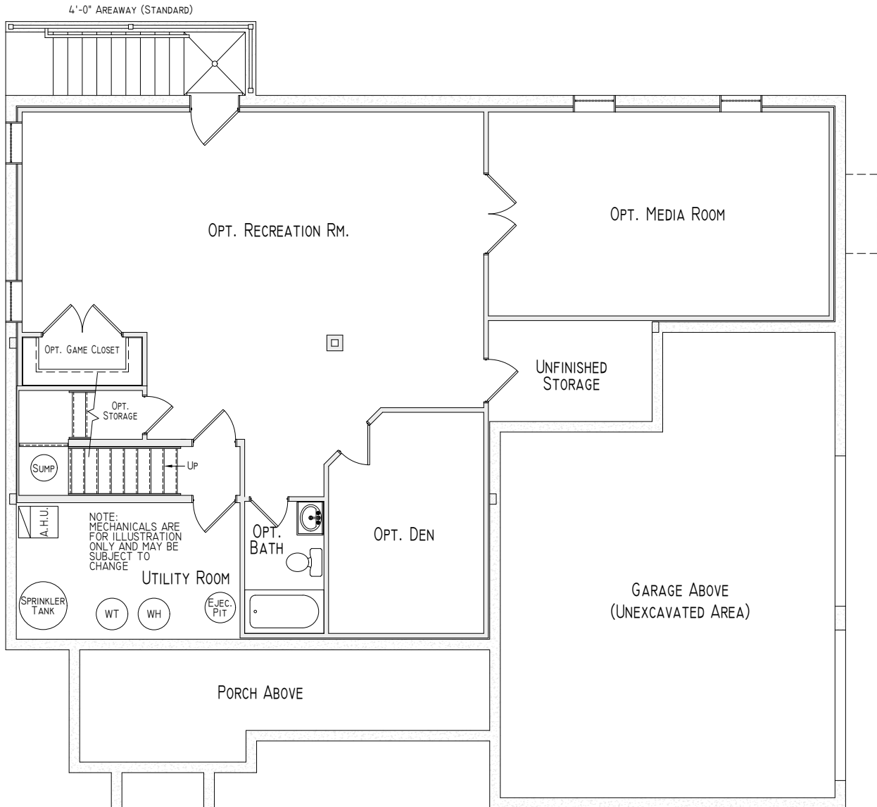
Foundation Plan
