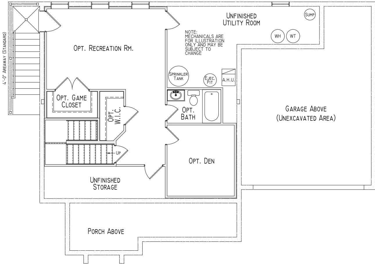
Foundation Plan
