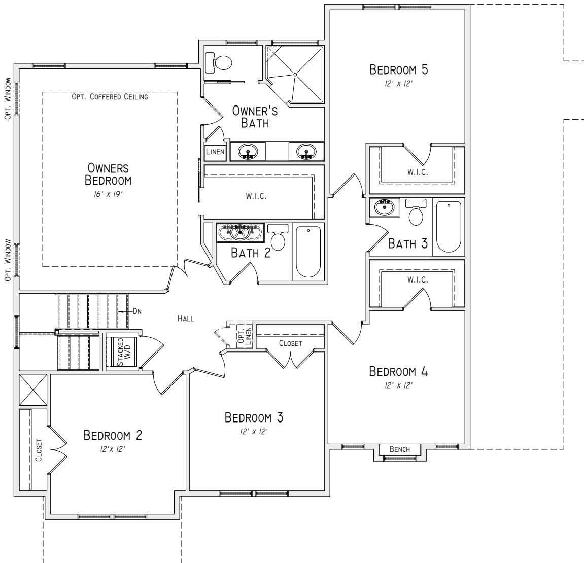
Second Floor Plan w/ Optional 5th Bedroom
