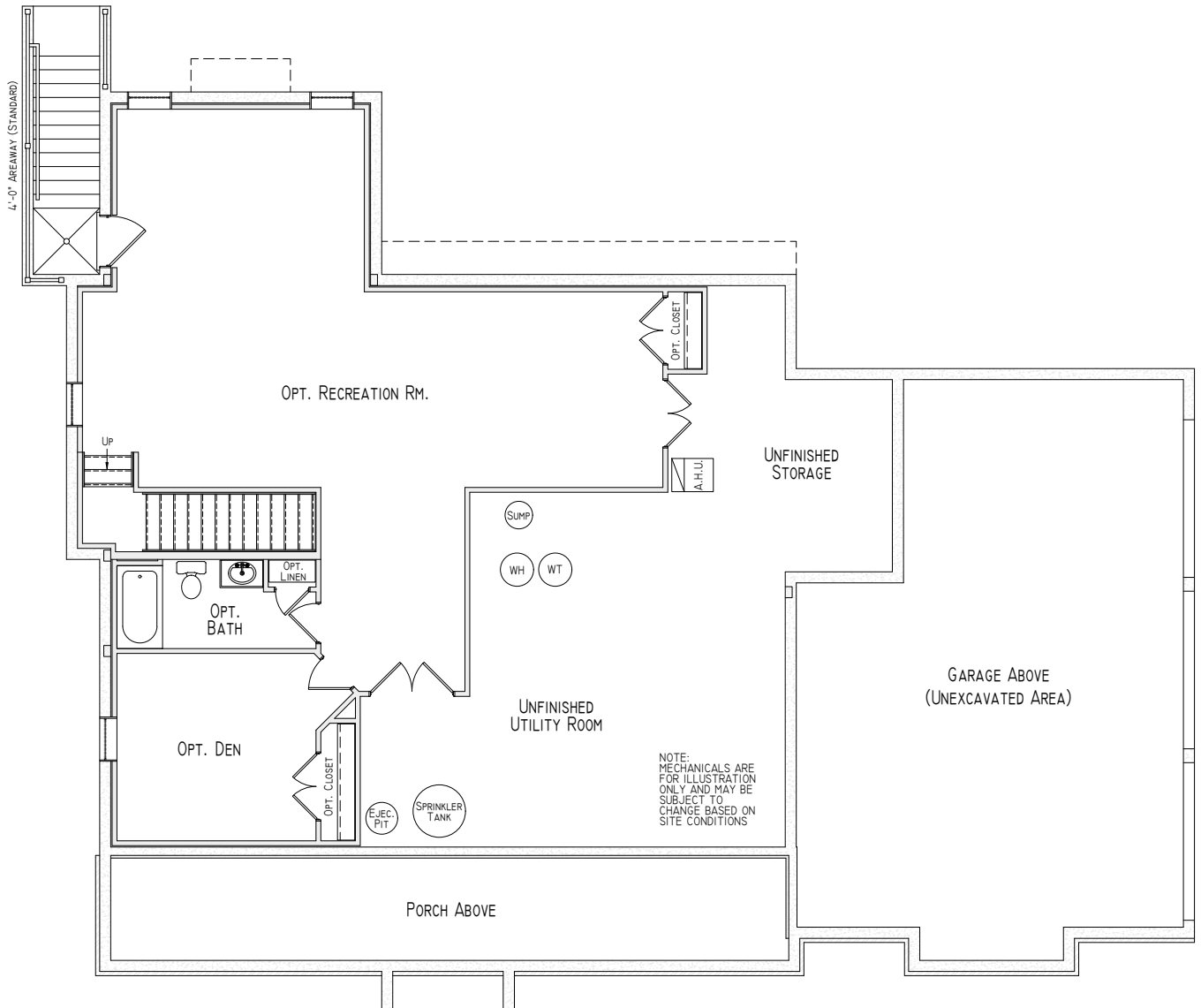
Foundation Plan
