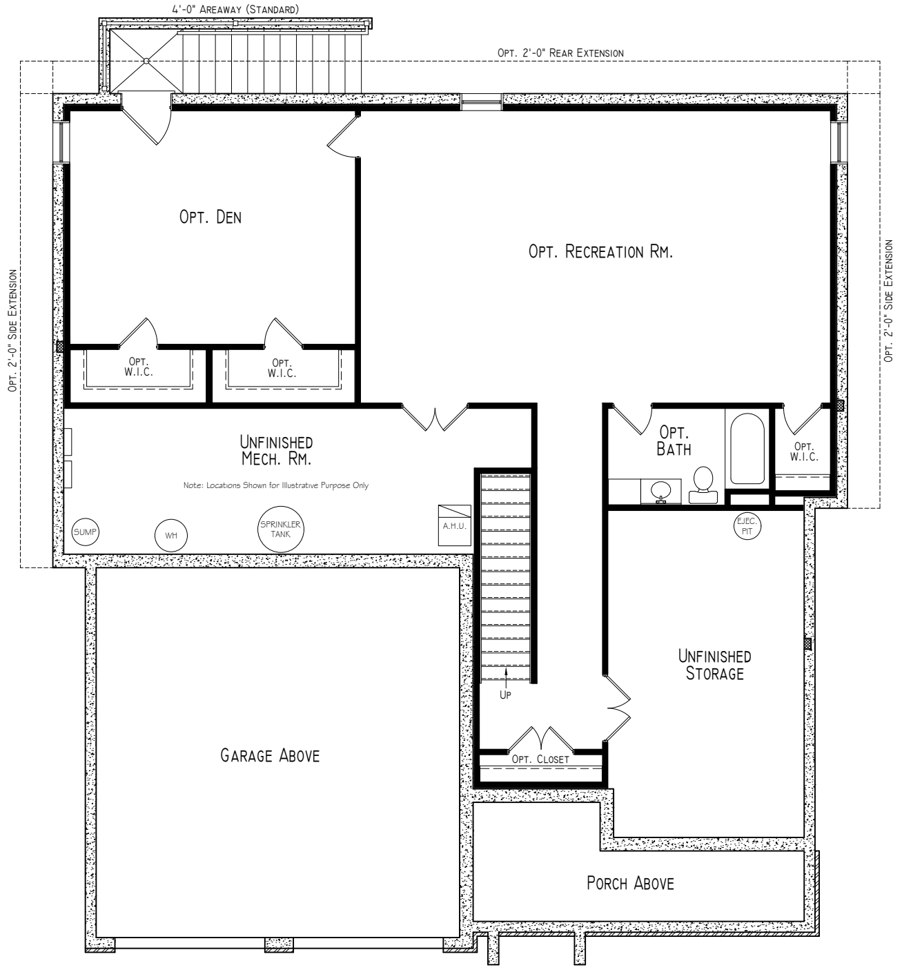
Foundation Plan
